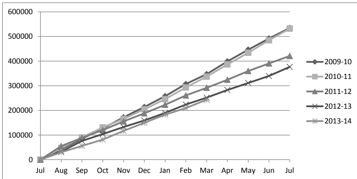
Figure 2: Cumulative Sewerage Discharge to Oxidation Ponds in cubic metres
